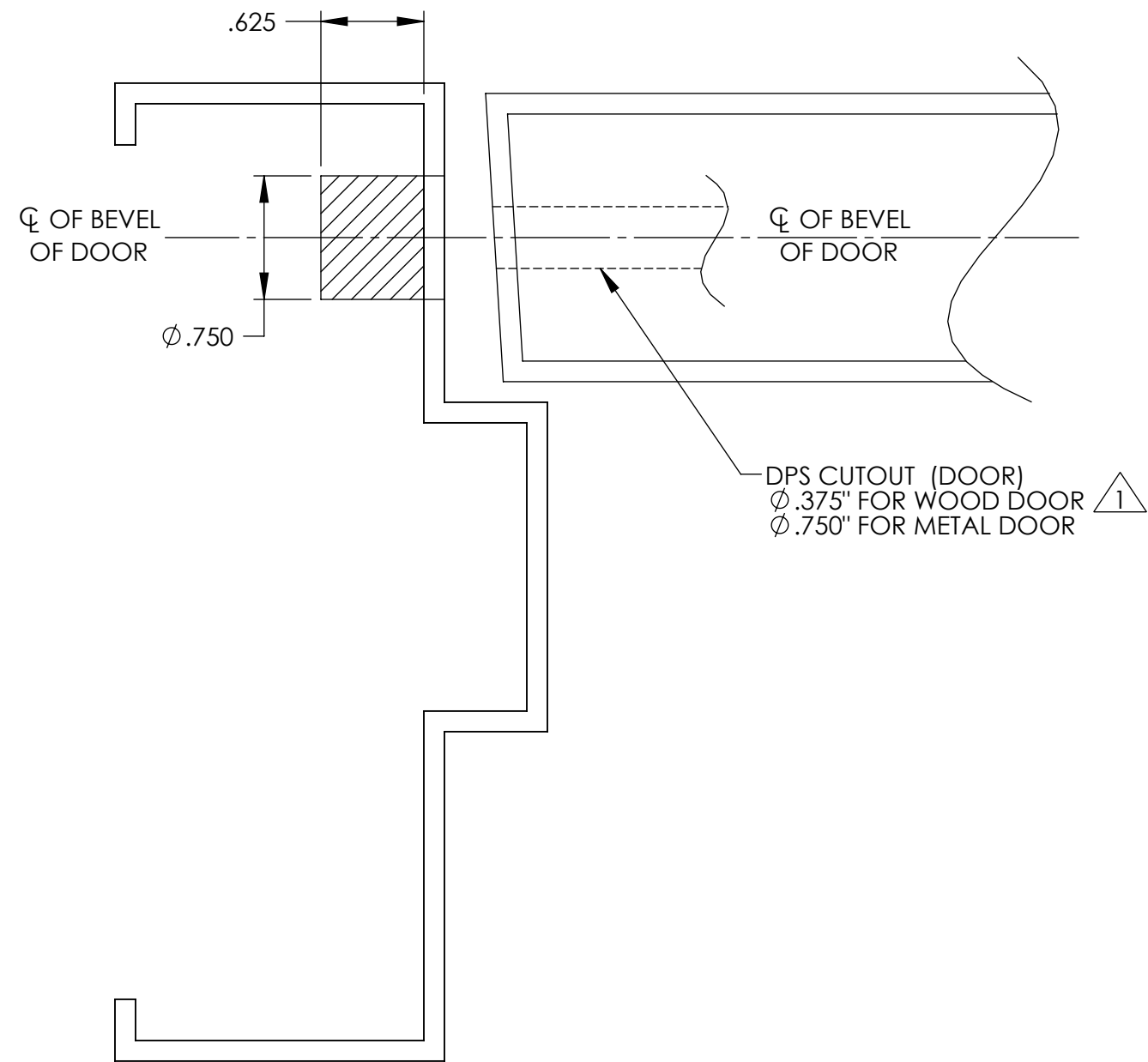
DOOR SHOWN IN CLOSED POSITION
