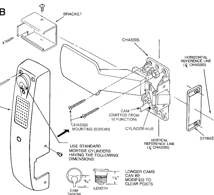
RIGHT HAND REVERSE BEVEL ILLUSTRATED
