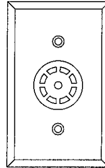
4380H - Horn only Face plate dimensions: 2 3/4" W x 4 1/2" H
