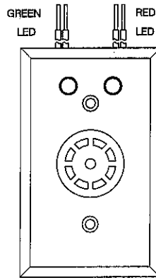
4380LH - Horn and LED's (Green and Red) Face plate dimensions: 2 3/4" W x 4 1/2" H
