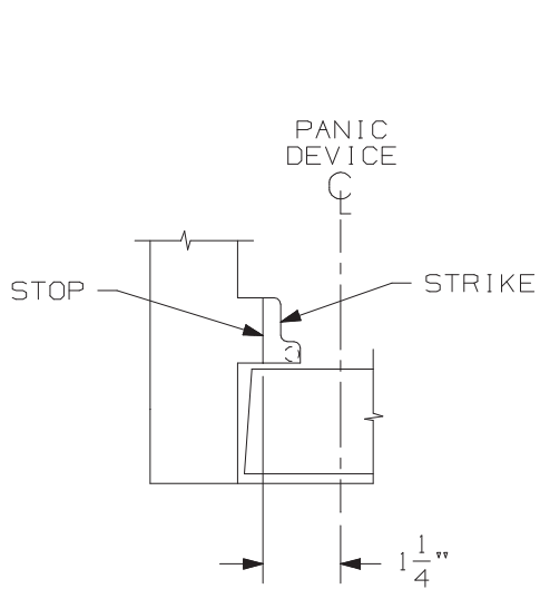
SINGLE DOOR TD35 OR TD36 SURFACE APPLIED STRIKE
