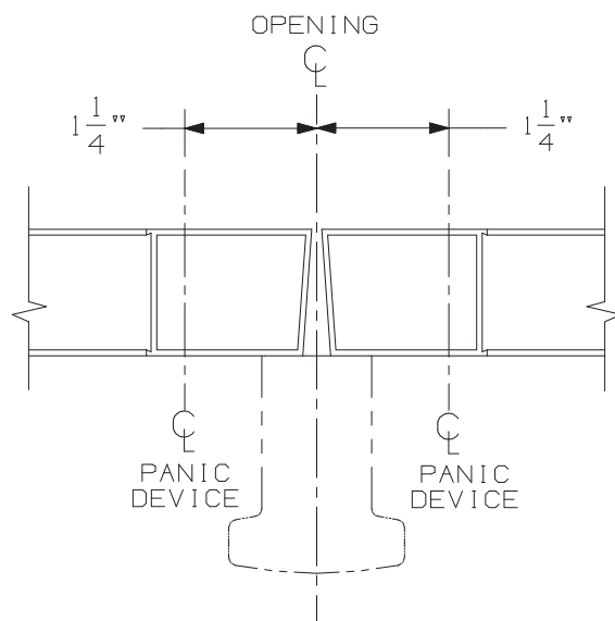
DOUBLE DOORS W/RM170 MULLION
