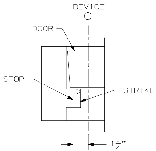
SINGLE DOOR SD35 OR SD36 SURFACE APPLIED STRIKE
