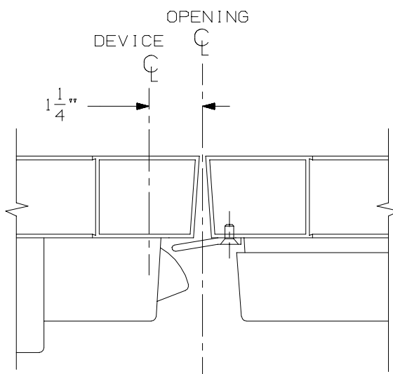
DOUBLE DOORS W/RD44 STRIKE
