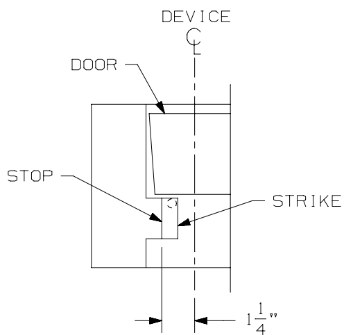
SINGLE DOOR TD35 SURFACE APPLIED STRIKE
