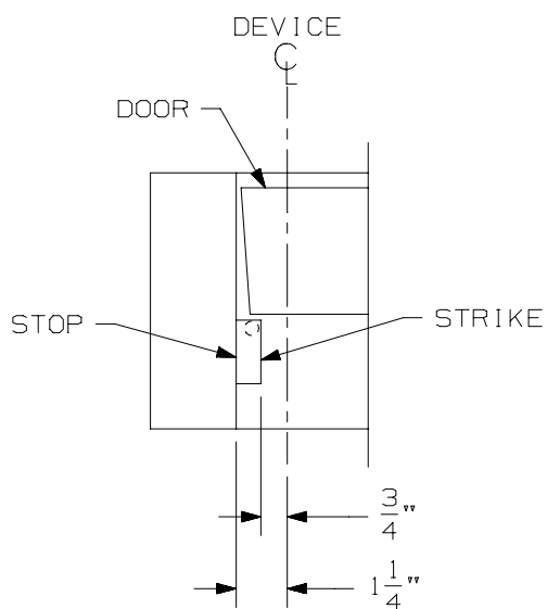
SINGLE DOOR TD35 MORTISED STRIKE
