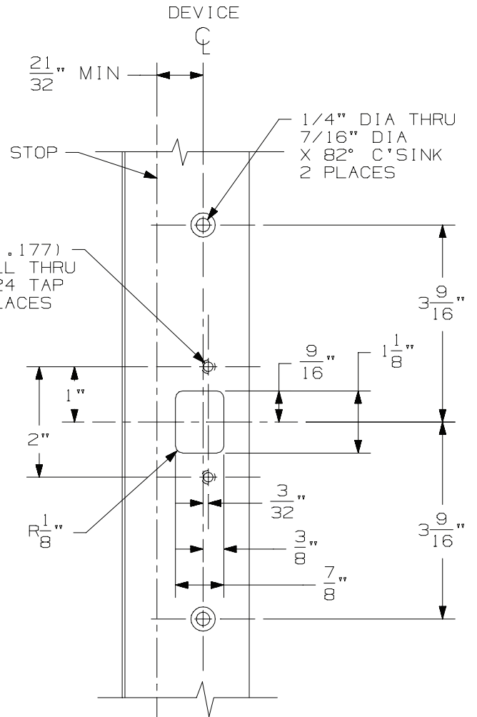
INSIDE FACE OF DOOR
