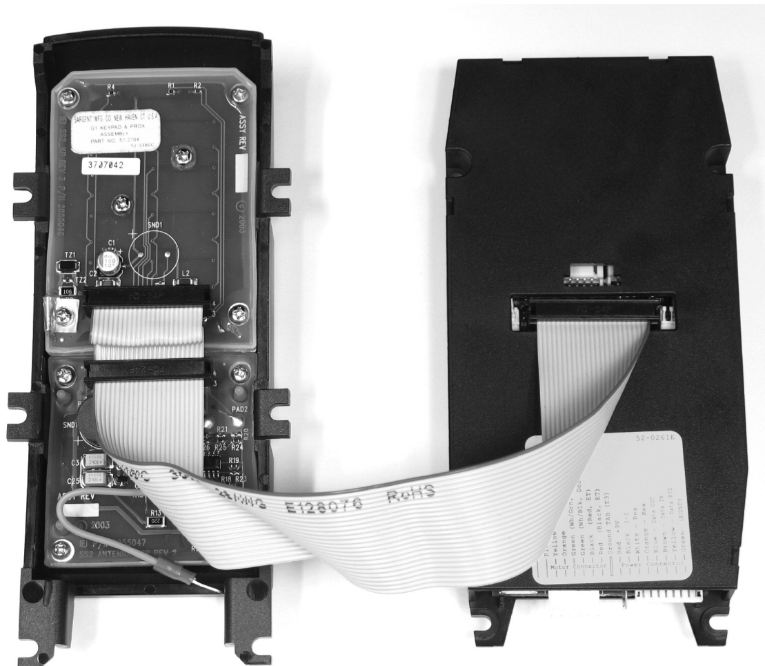
Figure 1 - New Ribbon Cable Orientation (install with cable exiting DOWN as shown)
