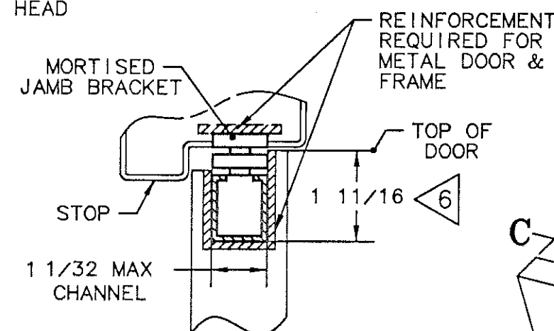
SECTIONAL VIEW WITH DOOR CLOSED
