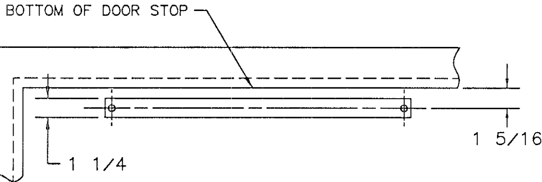
SWING CLEAR HINGE
