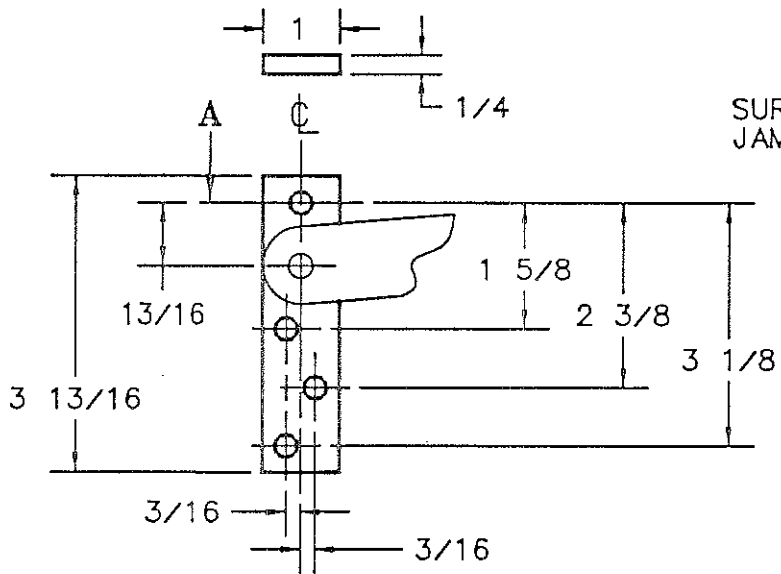
JAMB BRACKET DETAIL
