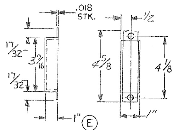
DETAIL OF STRIKE BOX
