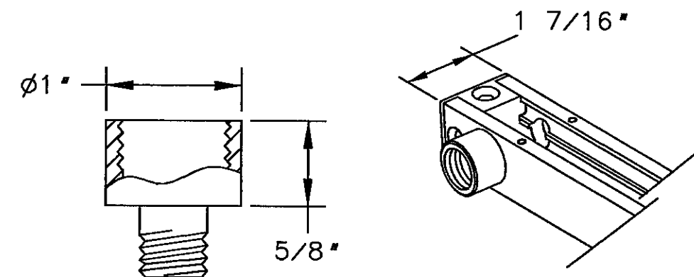
CONDUIT ADAPTER (6) (SHOWN INSTALLED ON SIDE OF CHANNEL)
