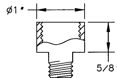
CONDUIT ADAPTER (SHOWN INSTALLED ON SIDE OF CHANNEL)
