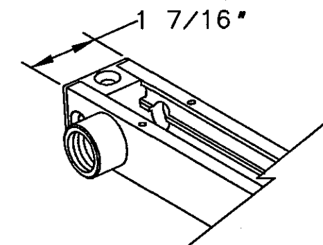
CONDUIT ADAPTER (SHOWN INSTALLED ON SIDE OF CHANNEL)
