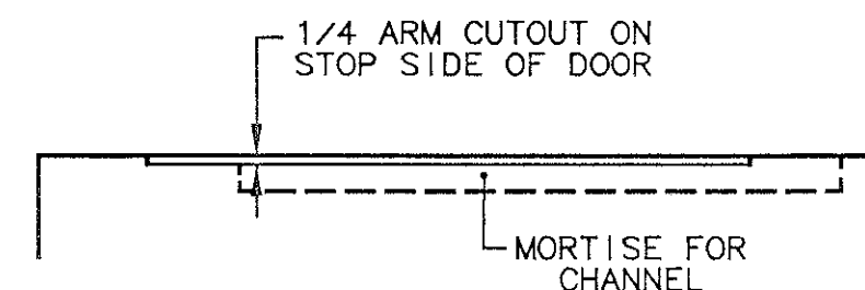
SECTIONAL VIEW WITH DOOR CLOSED
