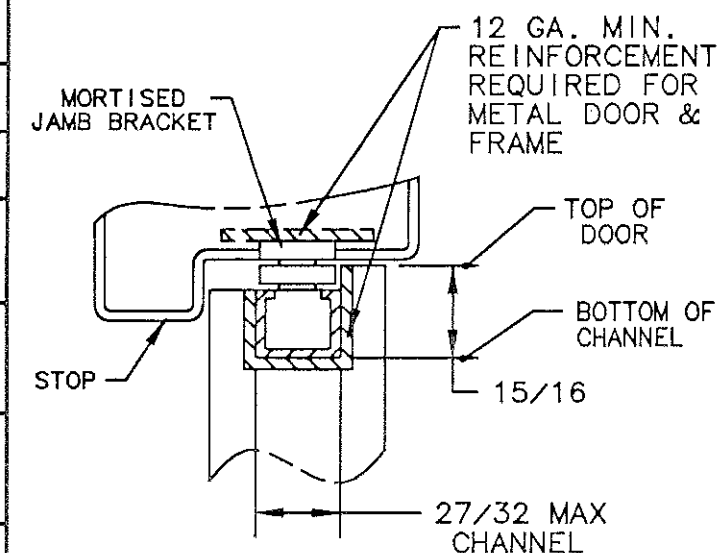
SECTIONAL VIEW WITH DOOR CLOSED
