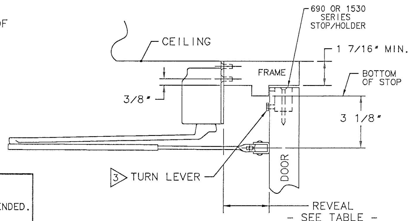
DOUBLE RABBETED FRAME (690 SHOWN)
