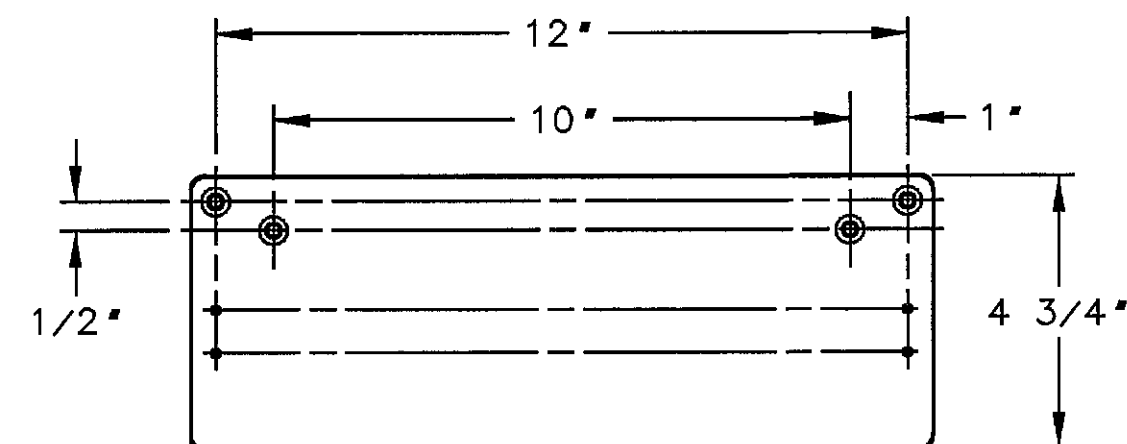
1331-D DROP PLATE DETAIL
