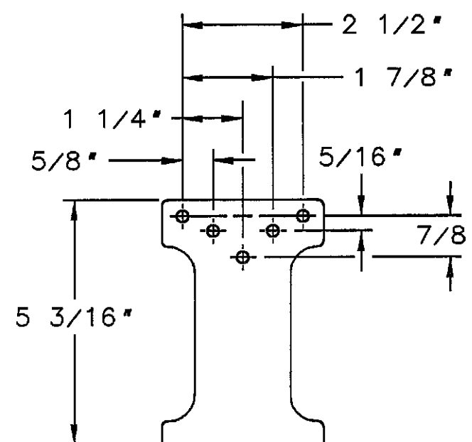
JPH9 FOOT BRACKET DETAIL
