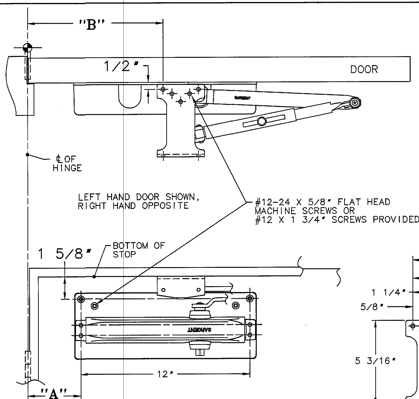
JPH9 FOOT BRACKET DETAIL
