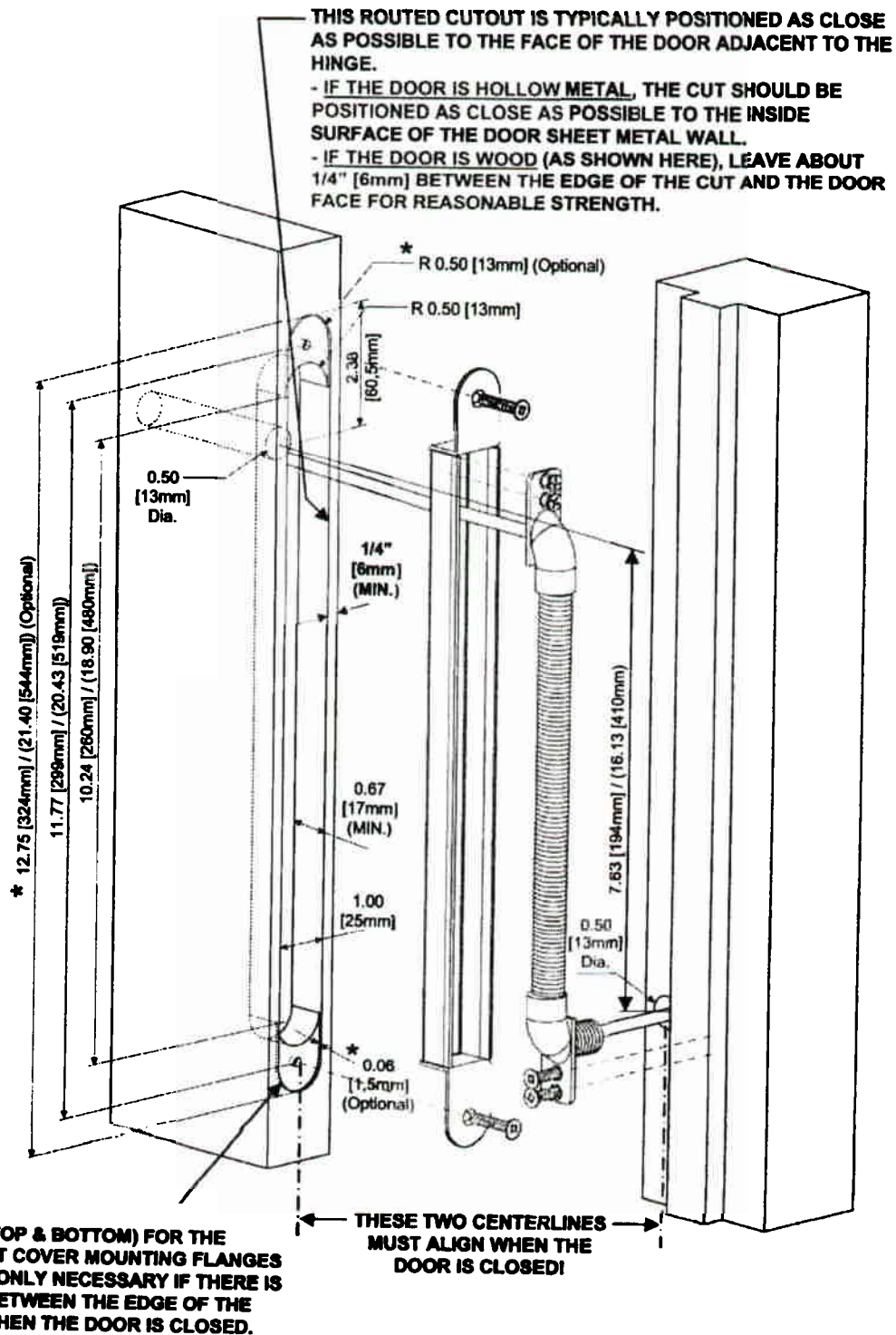
Figure 3: ROUTING DETAIL
